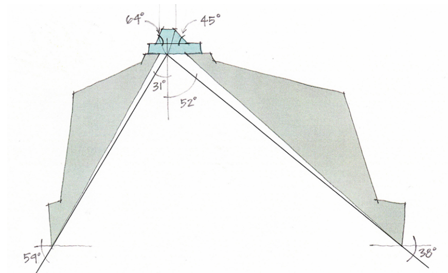
Figure 5: Typical container refraction analysis.
