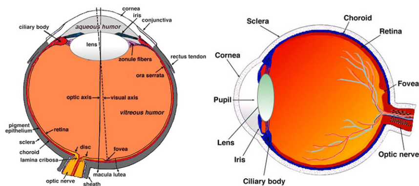
Figure 3: Sagittal horizontal and vertical sections of the adult human eye [3].
